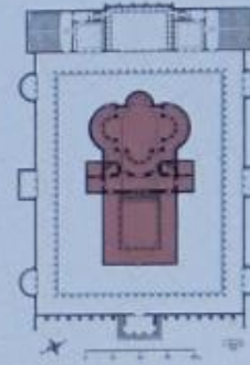
Βιβλιοθήκη Ἀδριανού, Κίτιον The courtyard of the palace of Septimius Severus, Library of Hadrian, Plan. The tetraconch church in the center of the courtyard.
