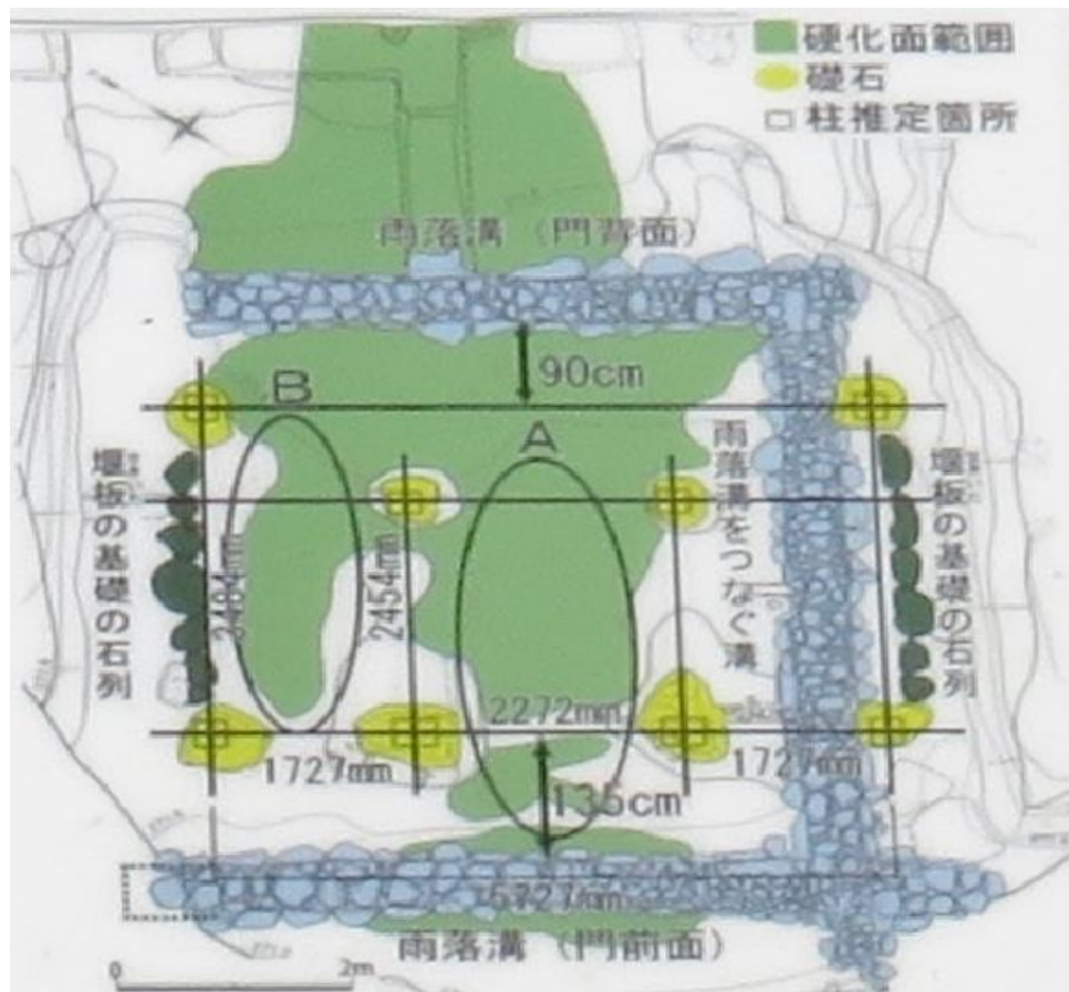
発掘調査時の郭馬出西虎口門 (図面)
